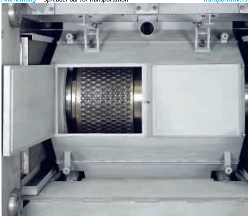
Roller housing
